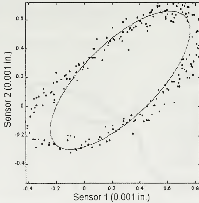
Figure 4.10 Ellipse fit for Heath's Method
